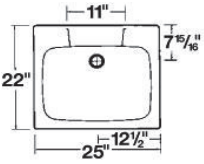
Combo dimensions: 25"W x 22"D x 35"H
